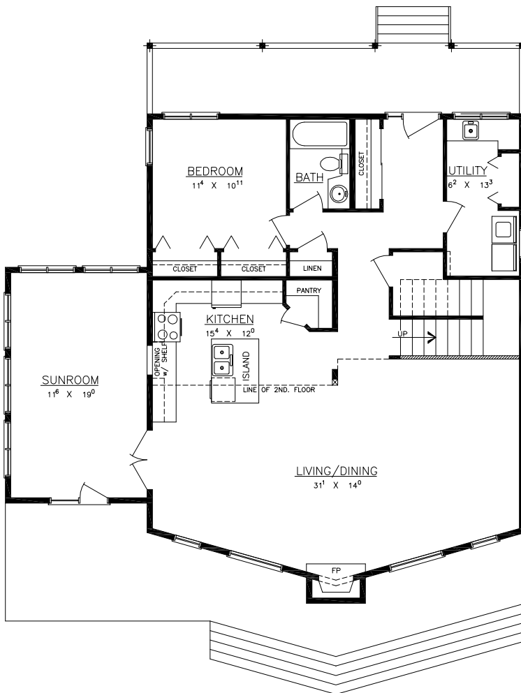
MAIN FLOOR
